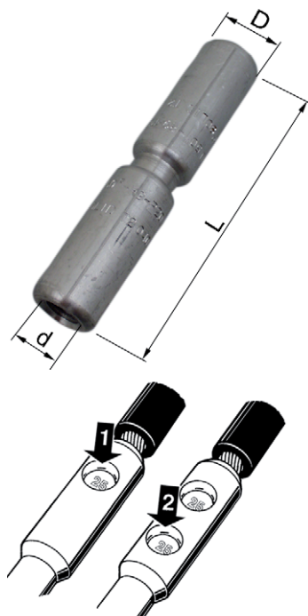
Crimp sequence.
