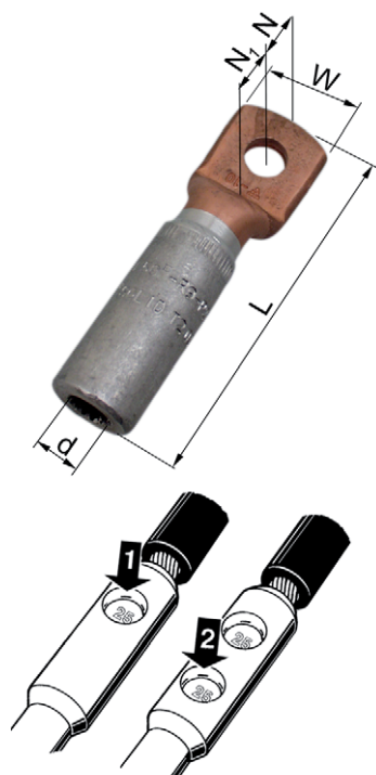
Crimp sequence.
