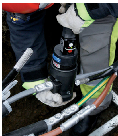
Crimping of Elpress Al through connector with crimp head V250.
