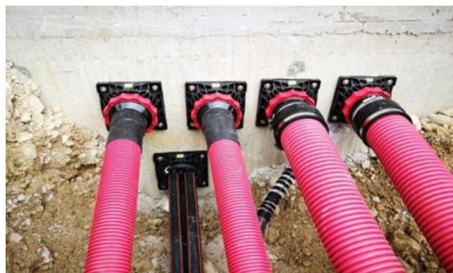
Vgrajene uvodnice HSI 150-DFK s sistemskimi pokrovi HSI 150-D110 KS, HSI 150-M168 WR in HSI 150-DG-3/24-54.
