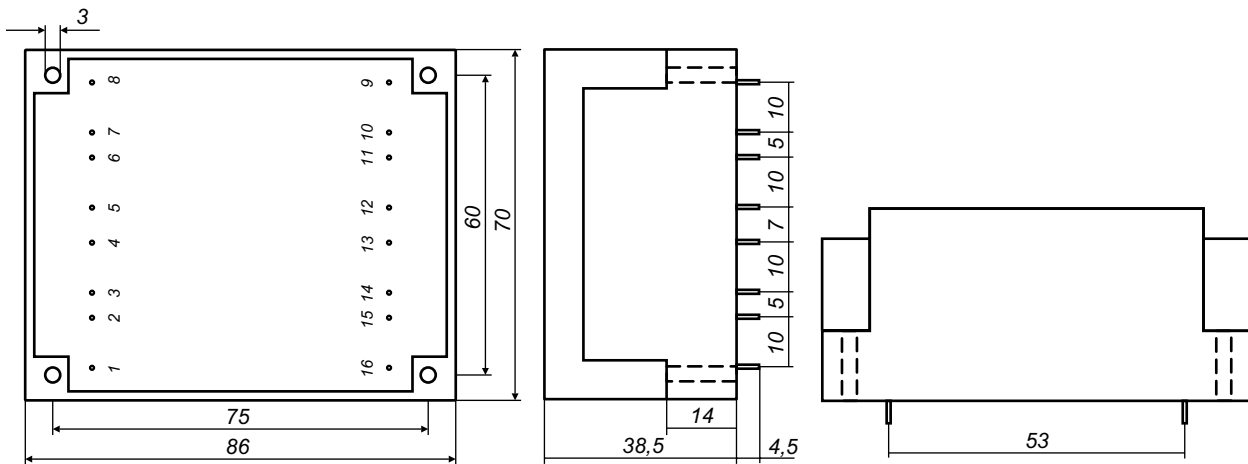
Dimensions in mm – View of pins
