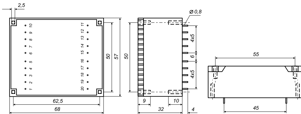
Dimensions in mm – View of pins
