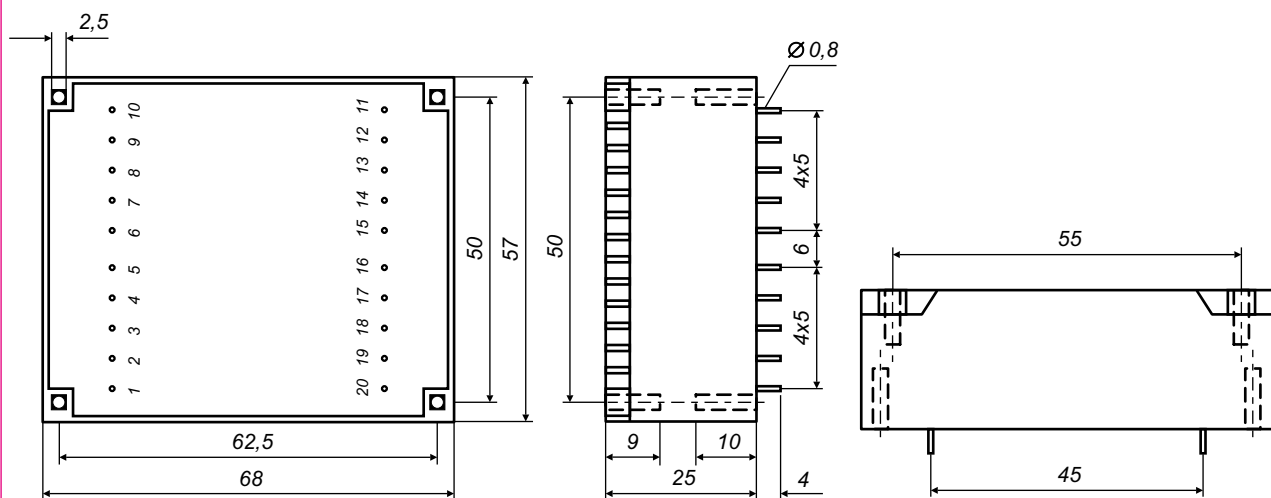
Dimensions in mm – View of pins
