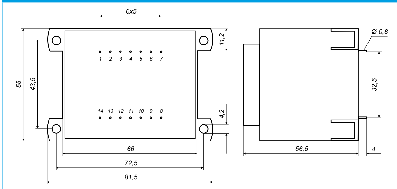
Dimensions in mm – View of pins
